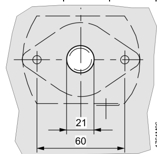
Drilling plan
